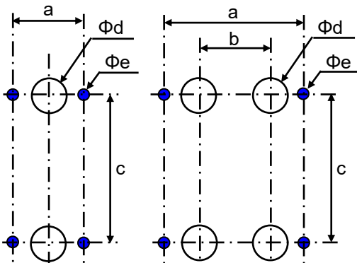
[ Fig. 3 ] [ Fig. 4 ] [ Panel boring dimensions ]
